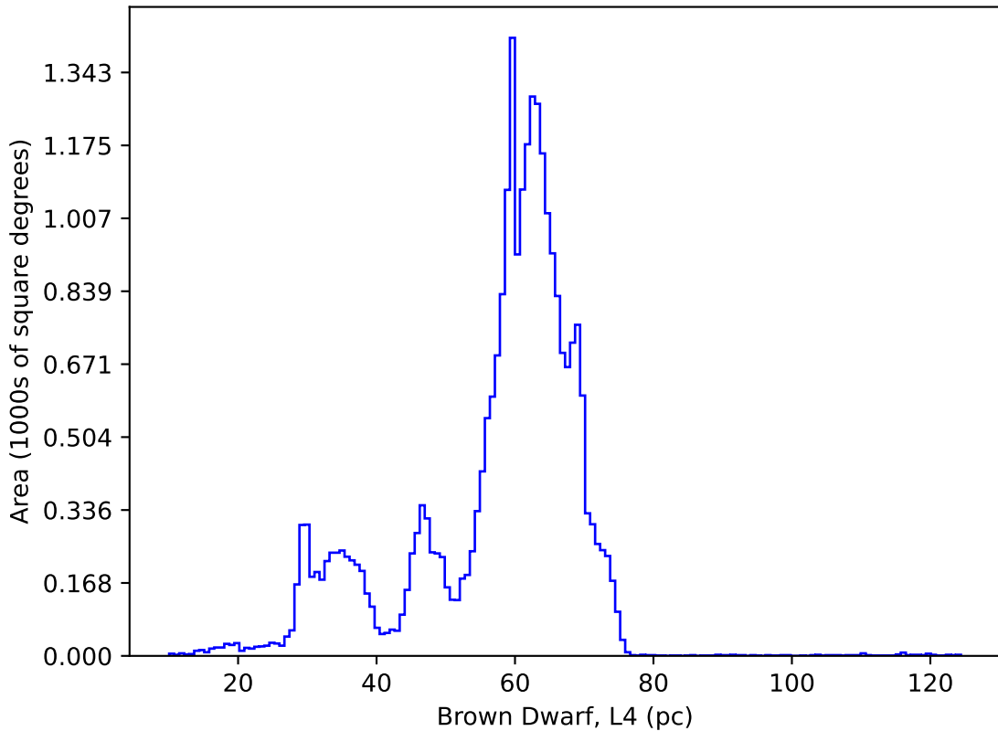
baseline_v3.2_10yrs : Brown Dwarf, L4
