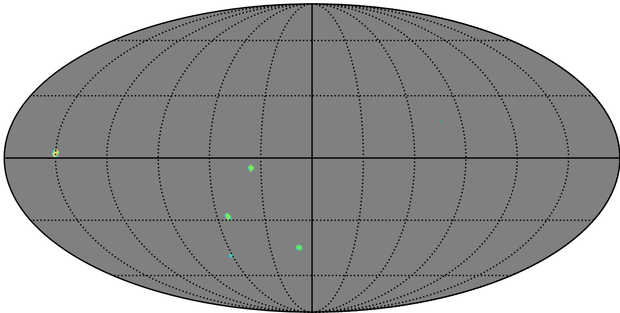
baseline_v3.2_10yrs z band: AGN_TimeLag_5_days
