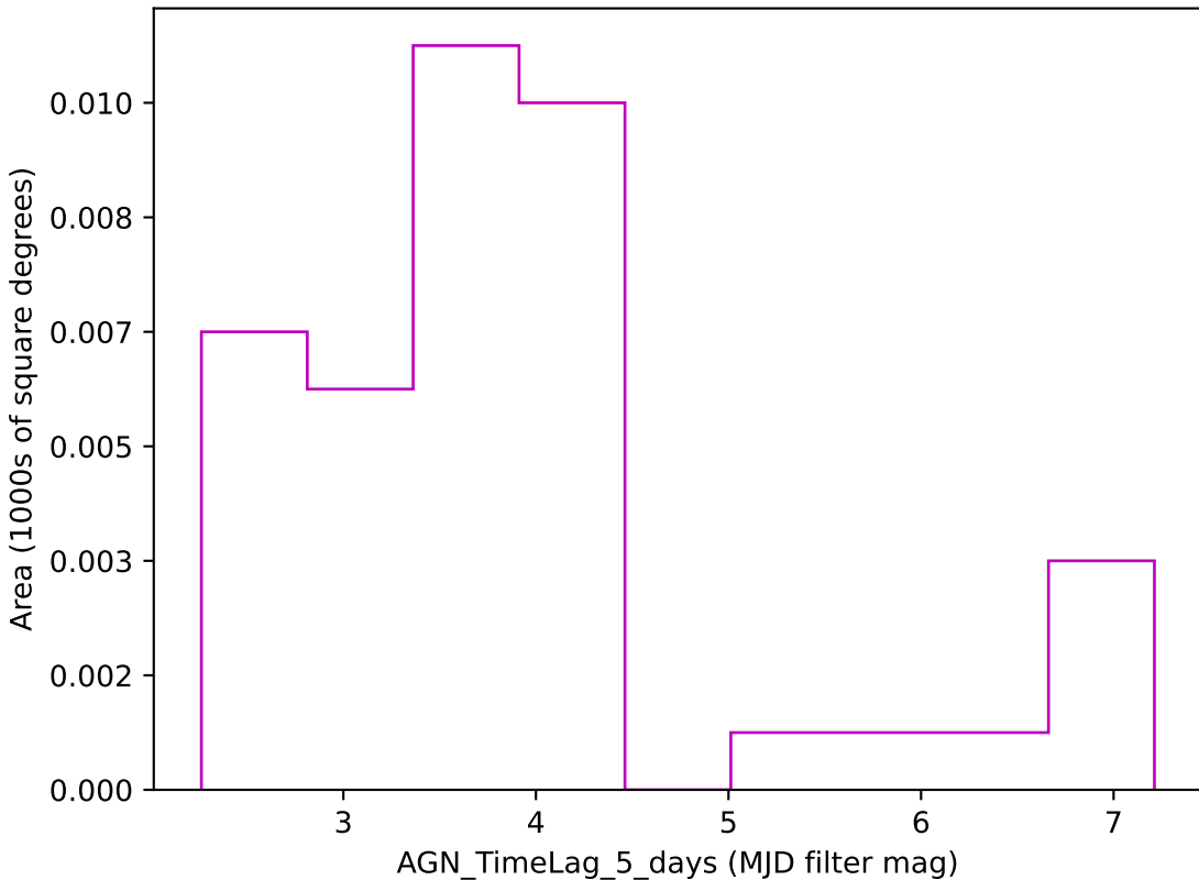
baseline_v3.2_10yrs z band: AGN_TimeLag_5_days
