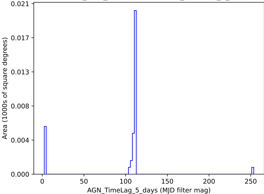
baseline_v3.2_10yrs y band: AGN_TimeLag_5_days
