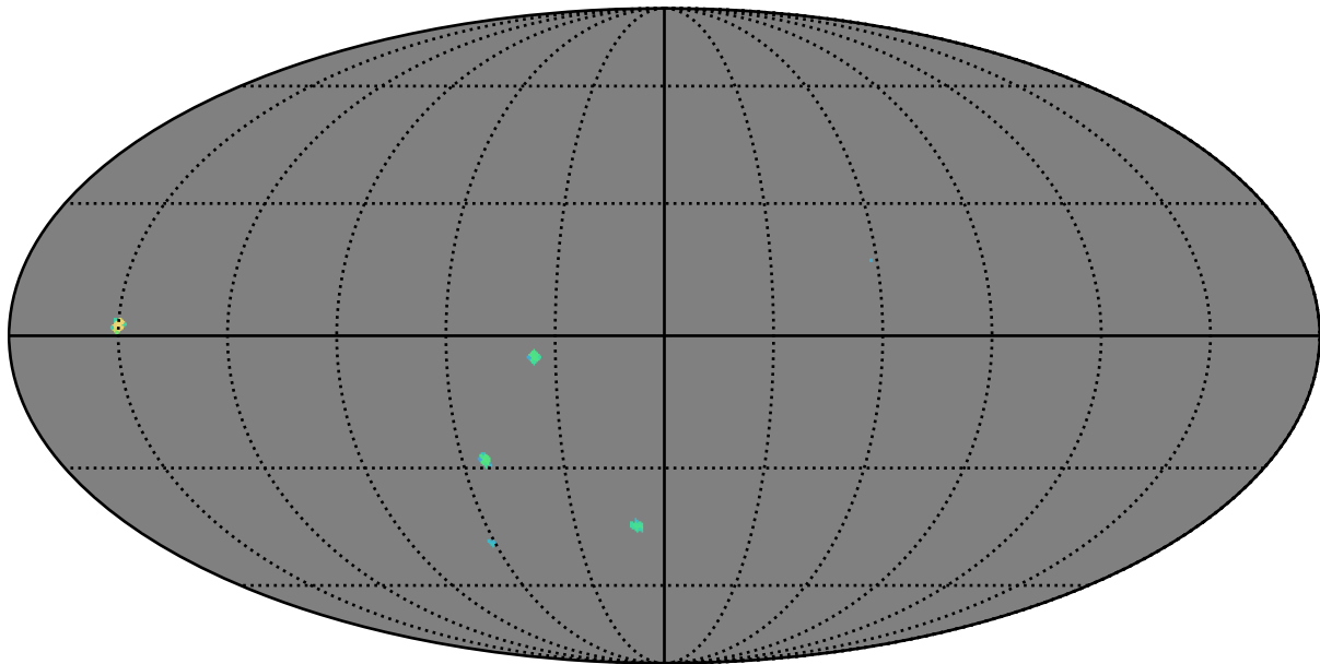
baseline_v3.2_10yrs r band: AGN_TimeLag_5_days
