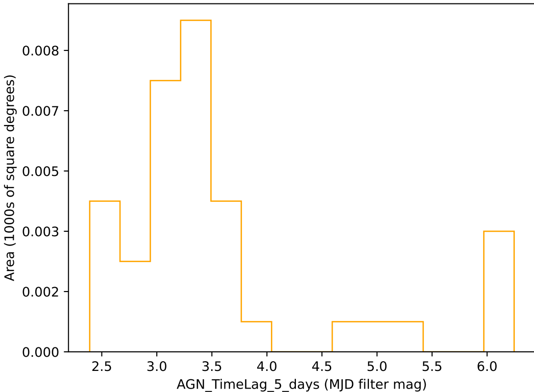
baseline_v3.2_10yrs r band: AGN_TimeLag_5_days
