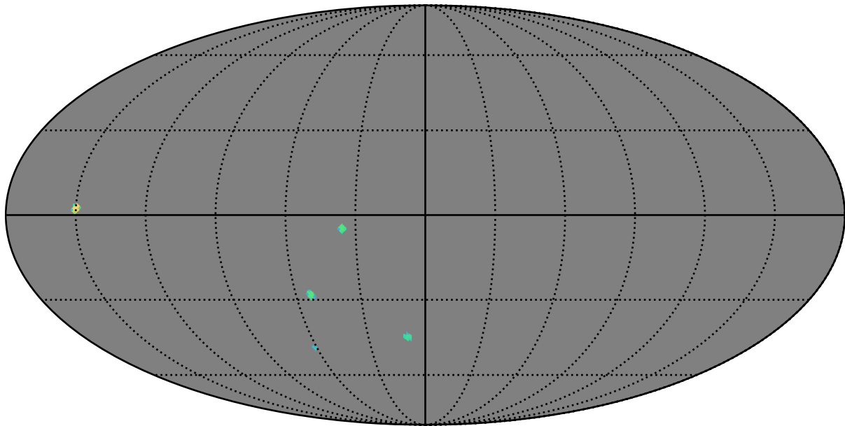
baseline_v3.2_10yrs i band: AGN_TimeLag_5_days
