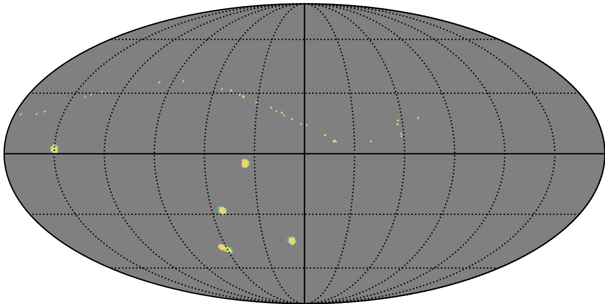
baseline_v3.2_10yrs all bands: AGN_TimeLag_5_days
