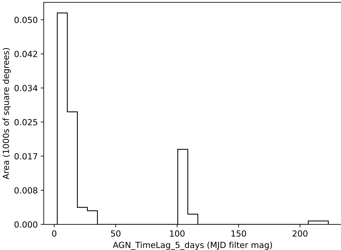
baseline_v3.2_10yrs all bands: AGN_TimeLag_5_days
