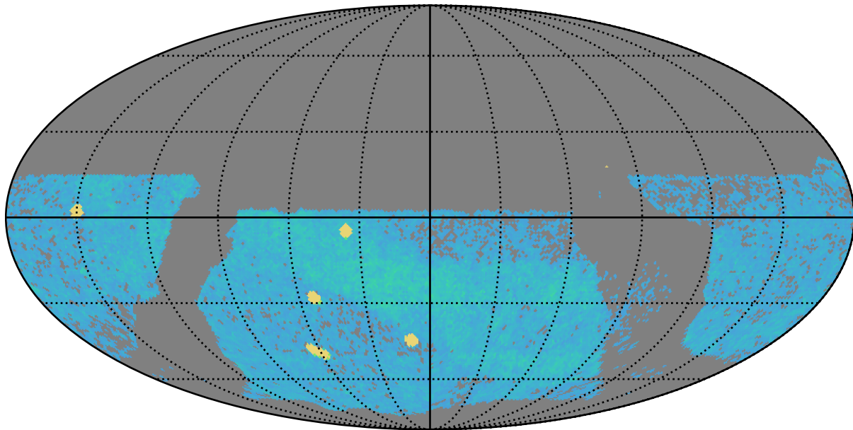
baseline_v3.2_10yrs z band: AGN_TimeLag_100_days
