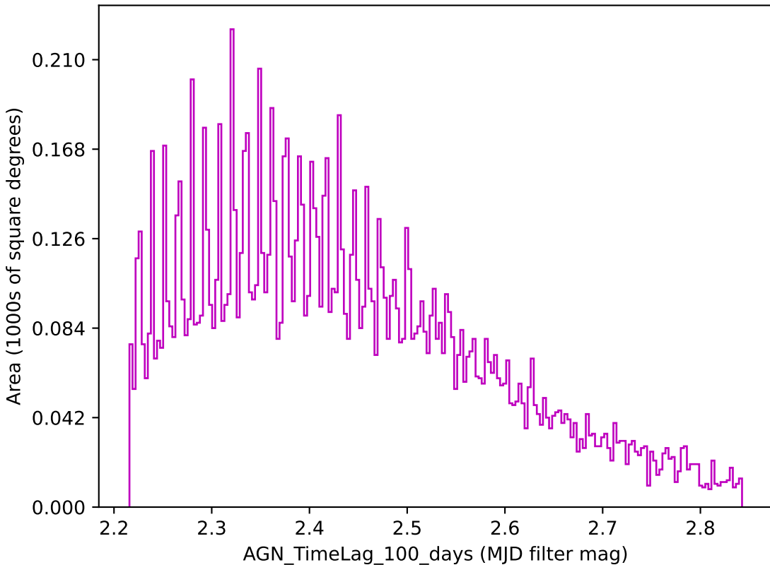
baseline_v3.2_10yrs z band: AGN_TimeLag_100_days
