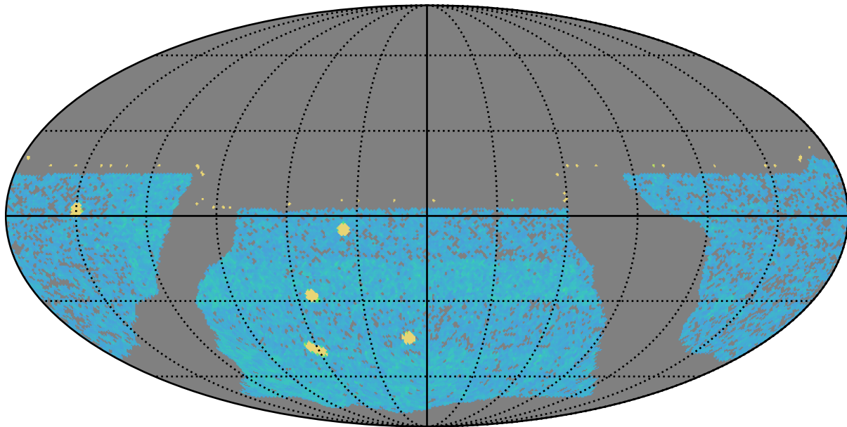
baseline_v3.2_10yrs y band: AGN_TimeLag_100_days
