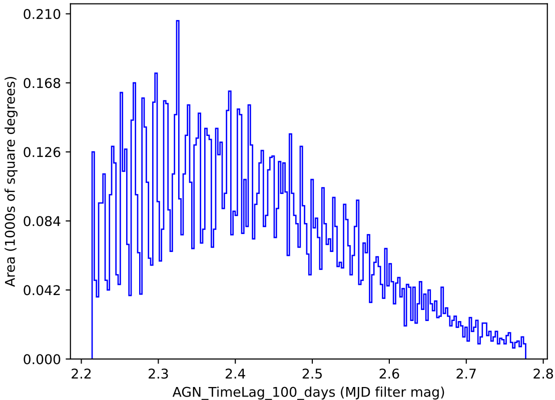
baseline_v3.2_10yrs y band: AGN_TimeLag_100_days
