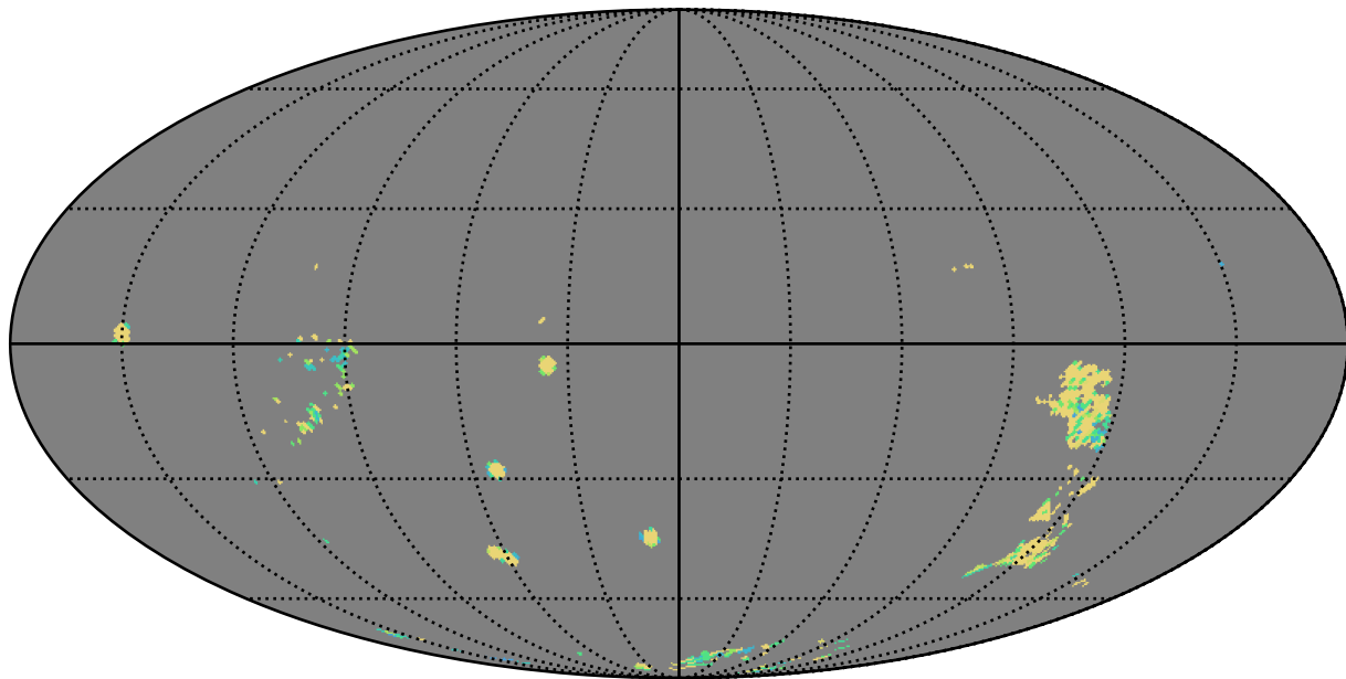
baseline_v3.2_10yrs u band: AGN_TimeLag_100_days
