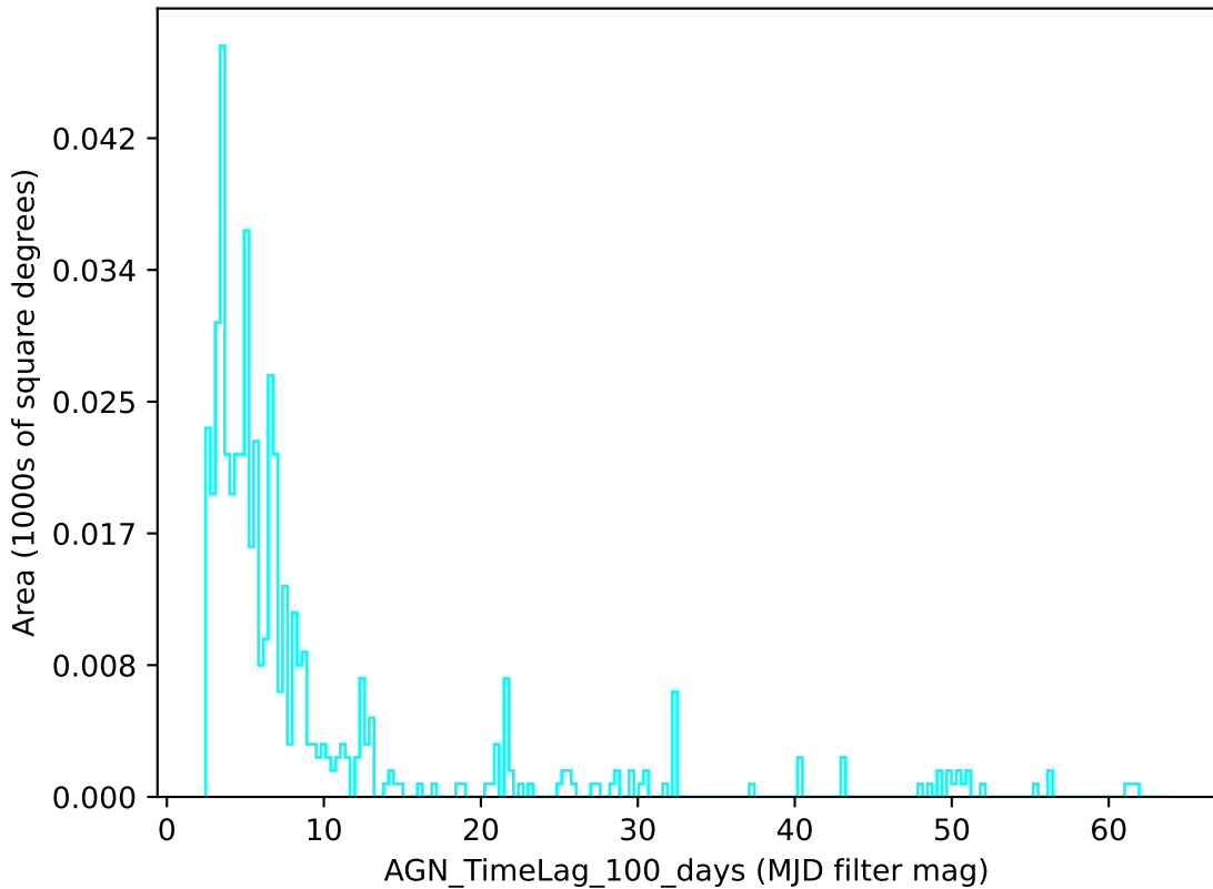
baseline_v3.2_10yrs u band: AGN_TimeLag_100_days
