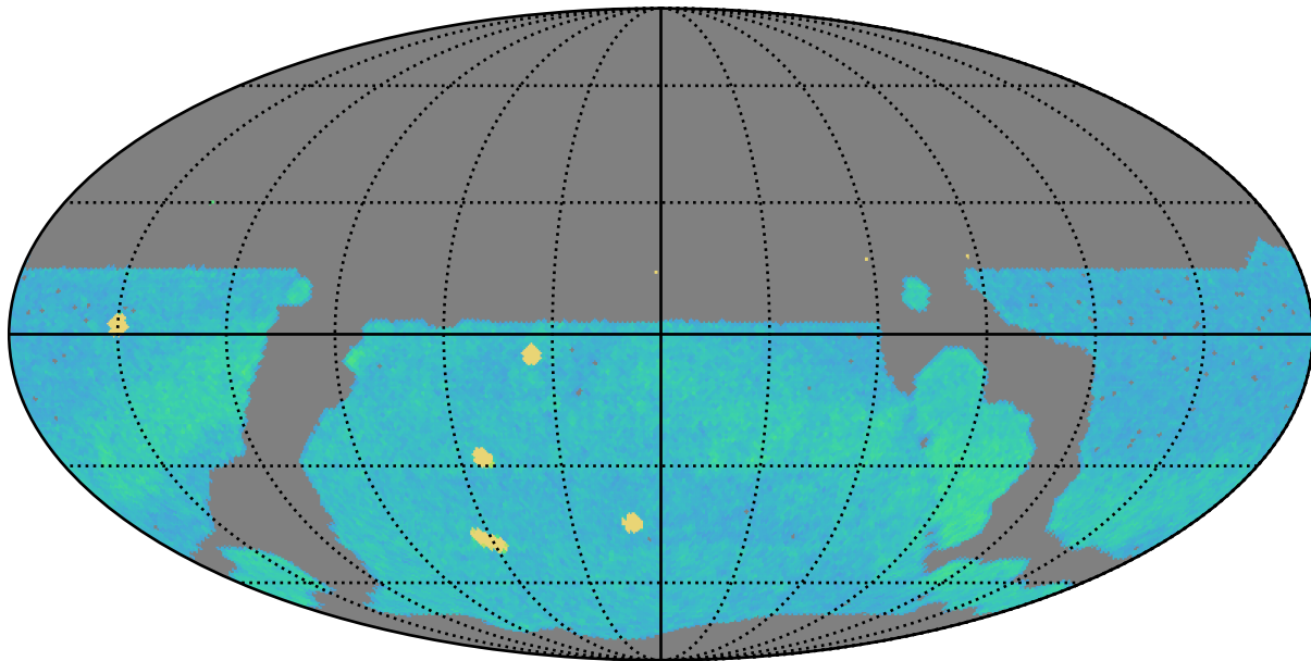
baseline_v3.2_10yrs r band: AGN_TimeLag_100_days
