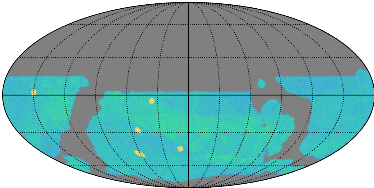
baseline_v3.2_10yrs i band: AGN_TimeLag_100_days
