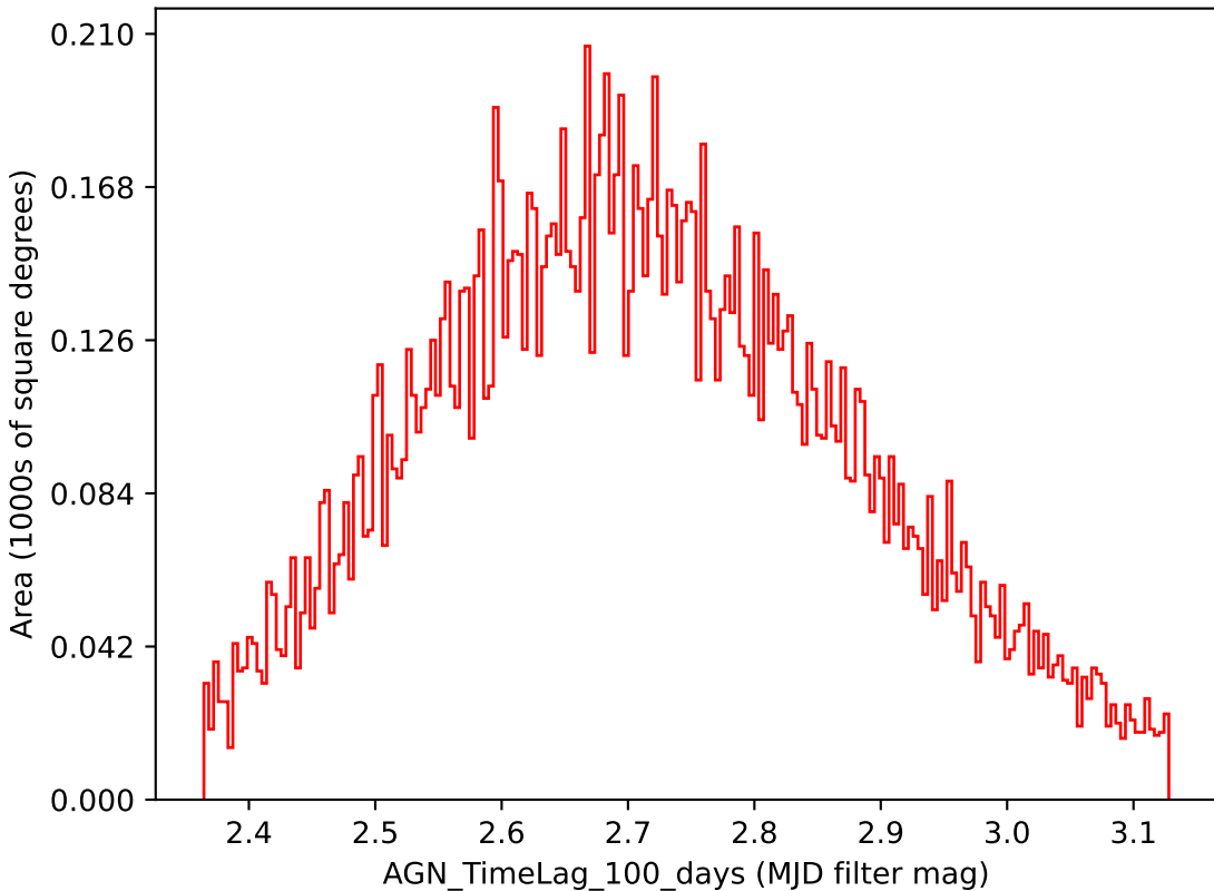
baseline_v3.2_10yrs i band: AGN_TimeLag_100_days
