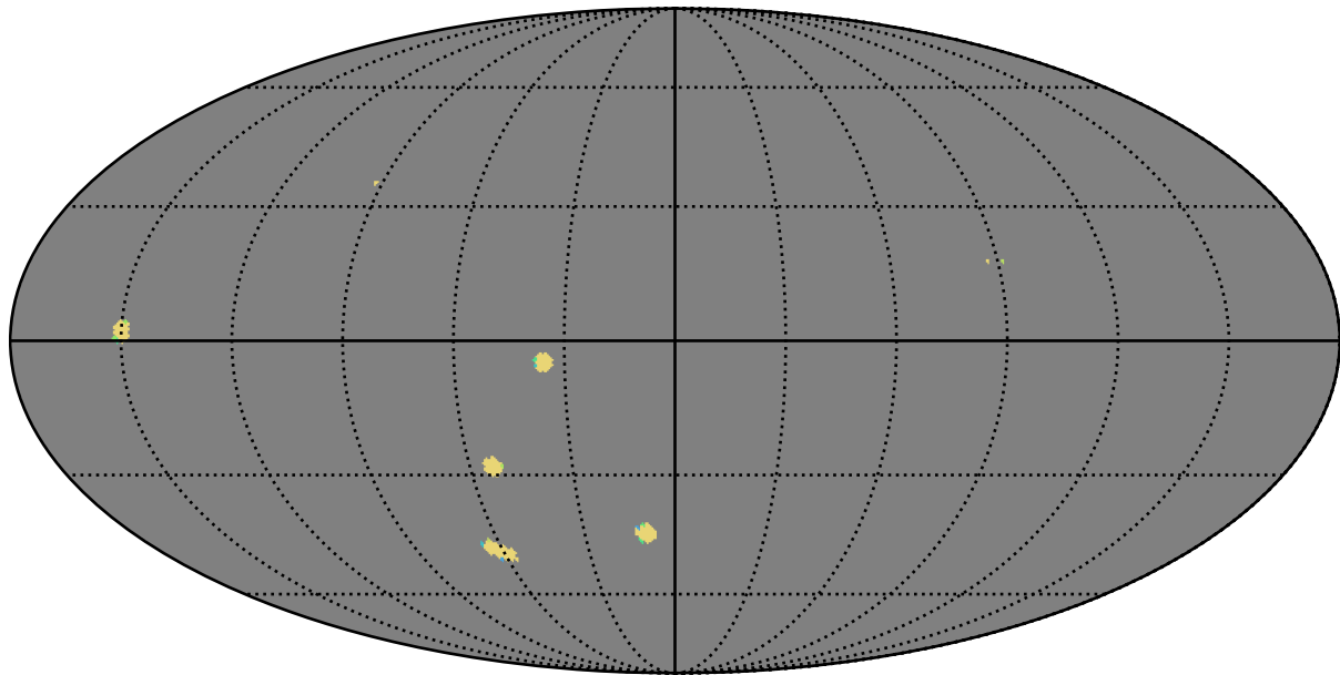
baseline_v3.2_10yrs g band: AGN_TimeLag_100_days
