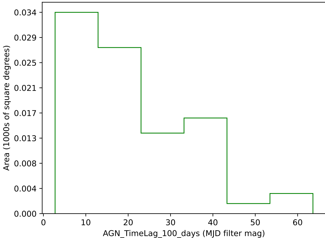
baseline_v3.2_10yrs g band: AGN_TimeLag_100_days
