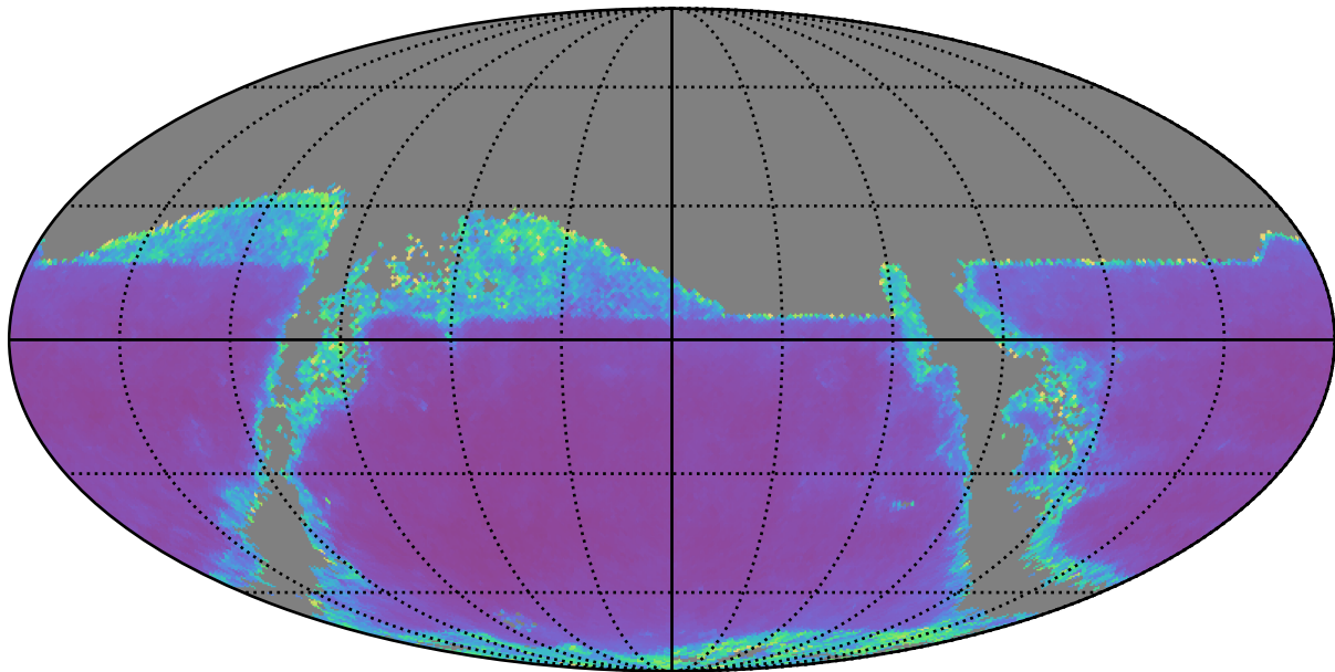
baseline_v3.2_10yrs z band: AGN SF_uncert
