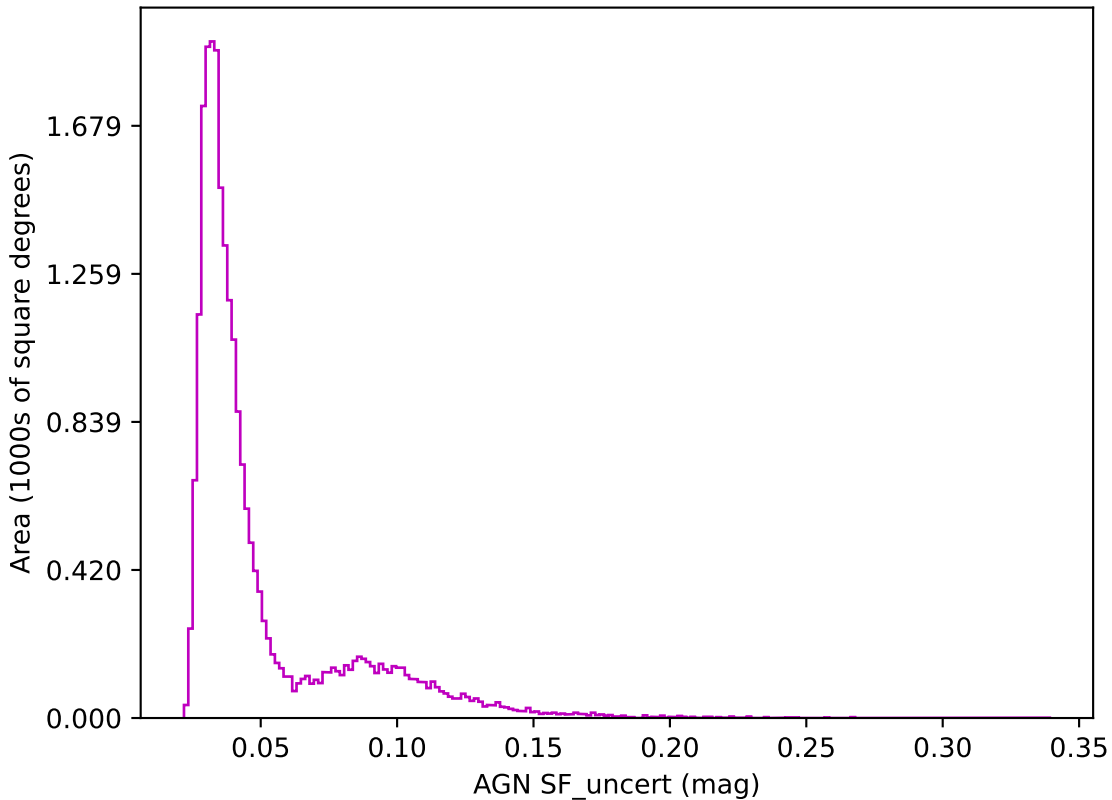
baseline_v3.2_10yrs z band: AGN SF_uncert
