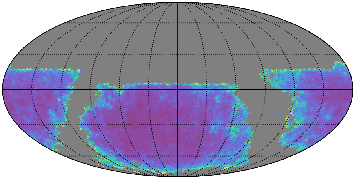
baseline_v3.2_10yrs u band: AGN SF_uncert
