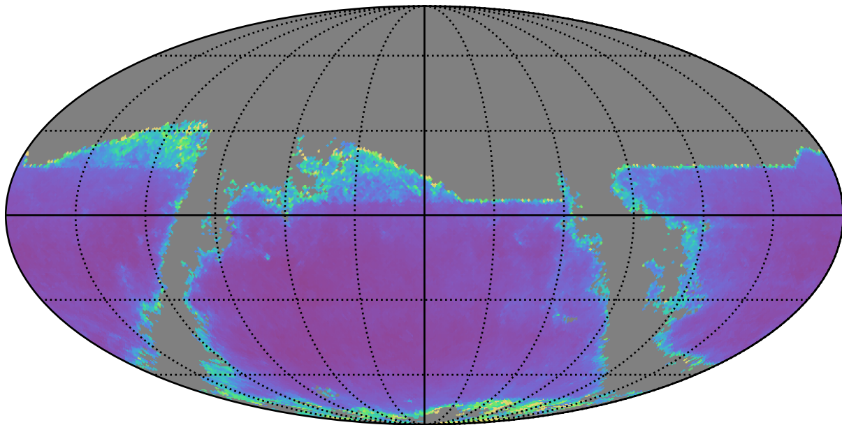
baseline_v3.2_10yrs r band: AGN SF_uncert
