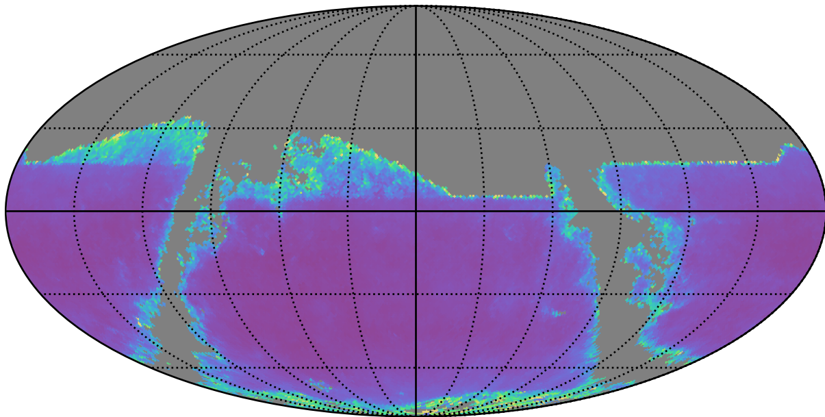
baseline_v3.2_10yrs i band: AGN SF_uncert
