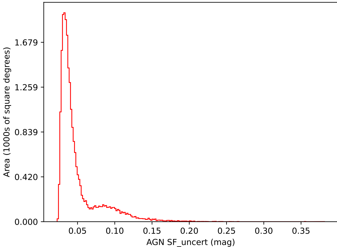
baseline_v3.2_10yrs i band: AGN SF_uncert
