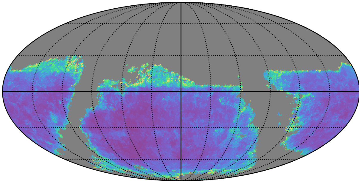
baseline_v3.2_10yrs g band: AGN SF_uncert
