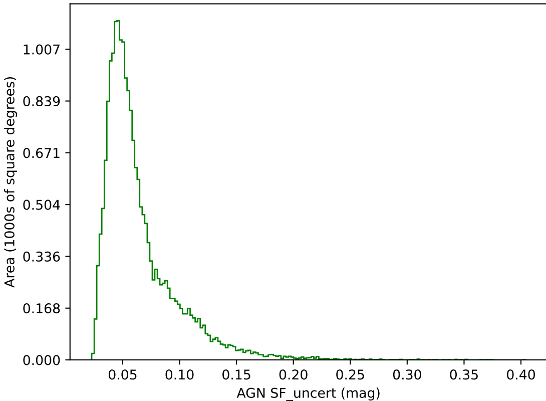
baseline_v3.2_10yrs g band: AGN SF_uncert
