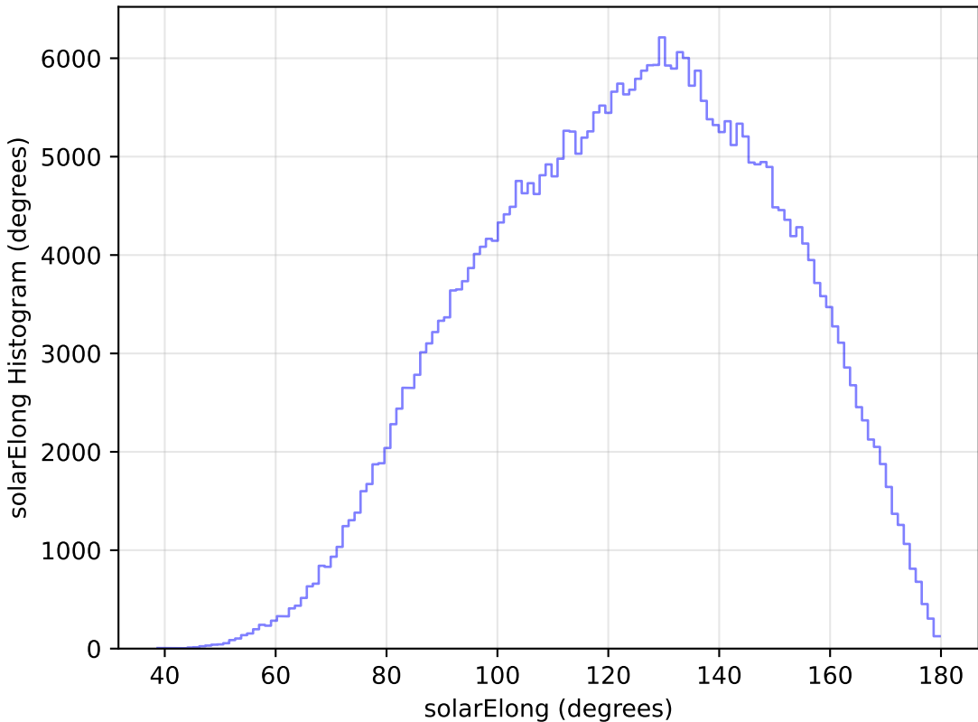
baseline_v3.2_10yrs WFD y band: solarElong Histogram
