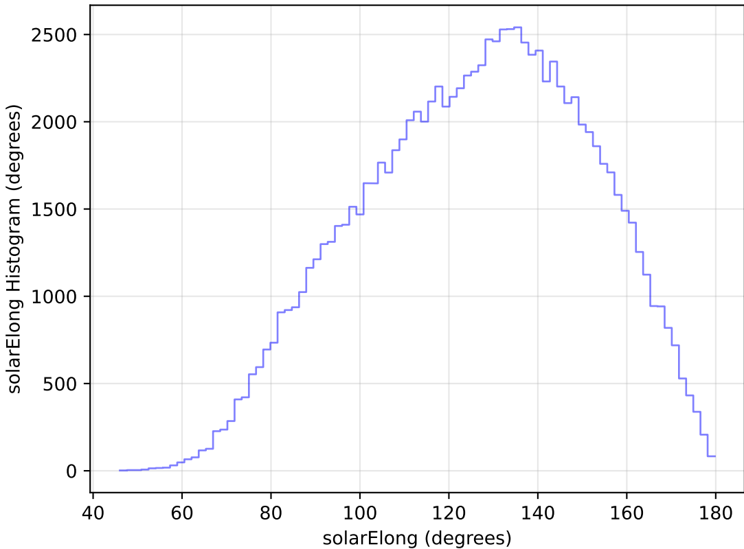
baseline_v3.2_10yrs WFD u band: solarElong Histogram
