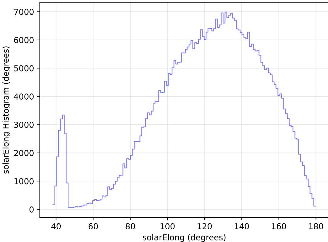
baseline_v3.2_10yrs WFD r band: solarElong Histogram
