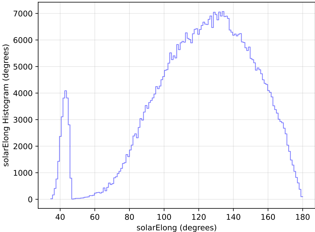
baseline_v3.2_10yrs WFD i band: solarElong Histogram
