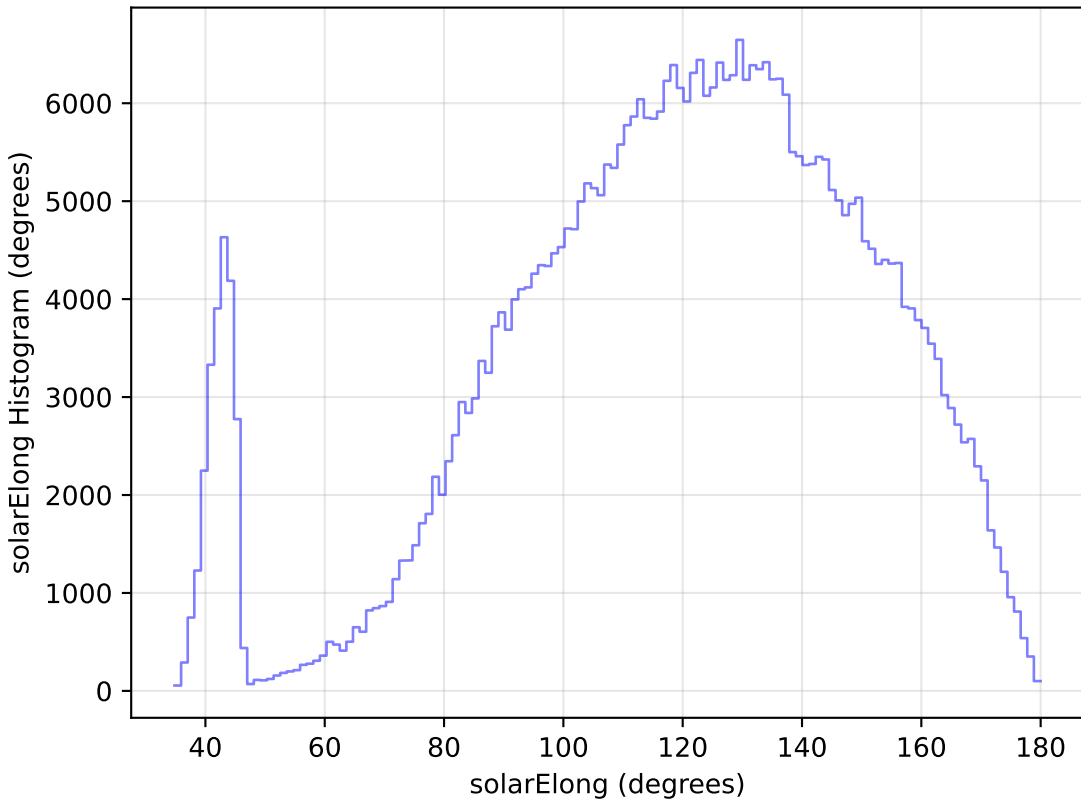
baseline_v3.2_10yrs All sky z band: solarElong Histogram
