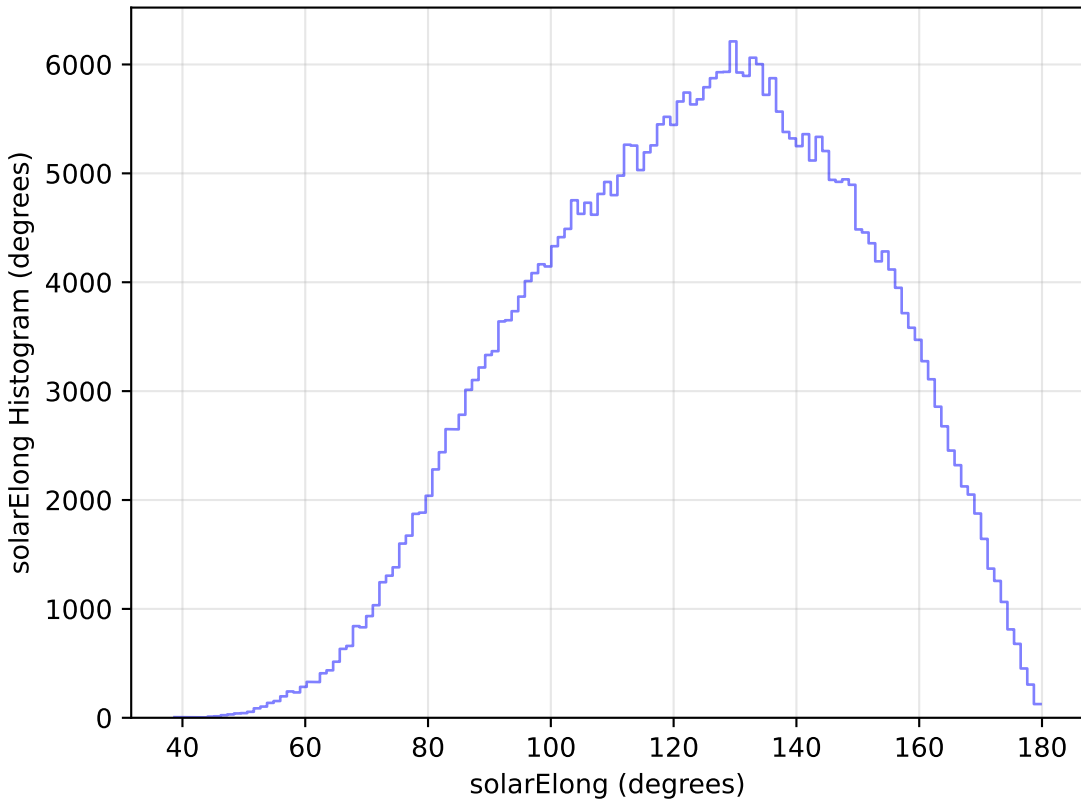
baseline_v3.2_10yrs All sky y band: solarElong Histogram
