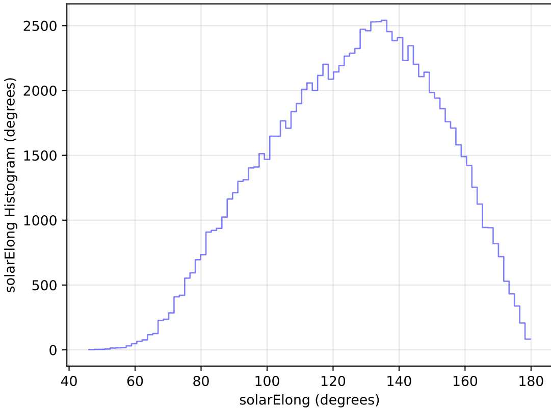
baseline_v3.2_10yrs All sky u band: solarElong Histogram
