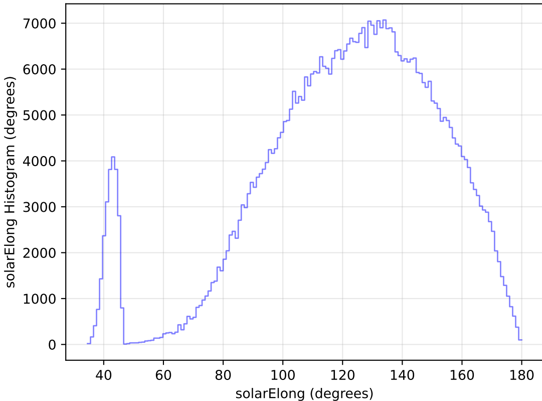
baseline_v3.2_10yrs All sky i band: solarElong Histogram
