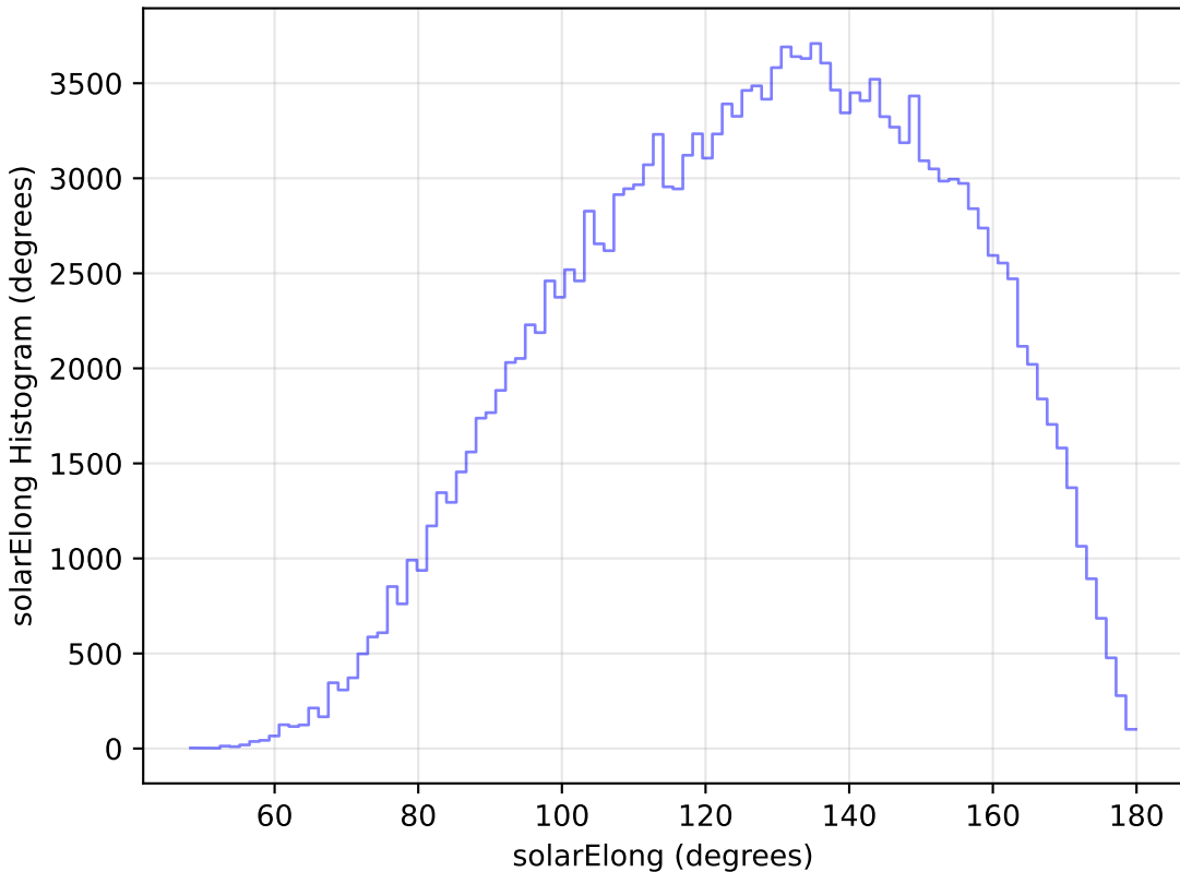
baseline_v3.2_10yrs All sky g band: solarElong Histogram
