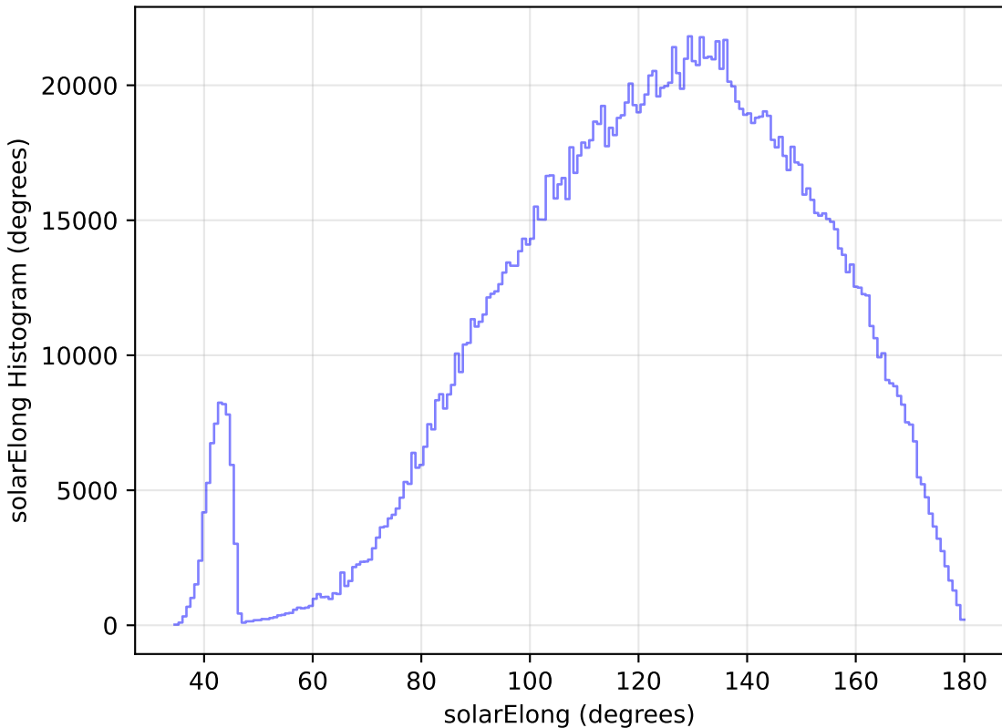
baseline_v3.2_10yrs All sky all bands: solarElong Histogram
