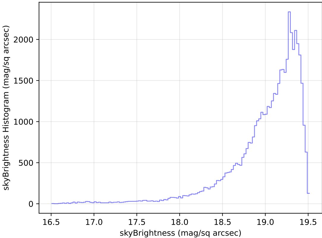
baseline_v3.2_10yrs Yr 1 z band: skyBrightness Histogram
