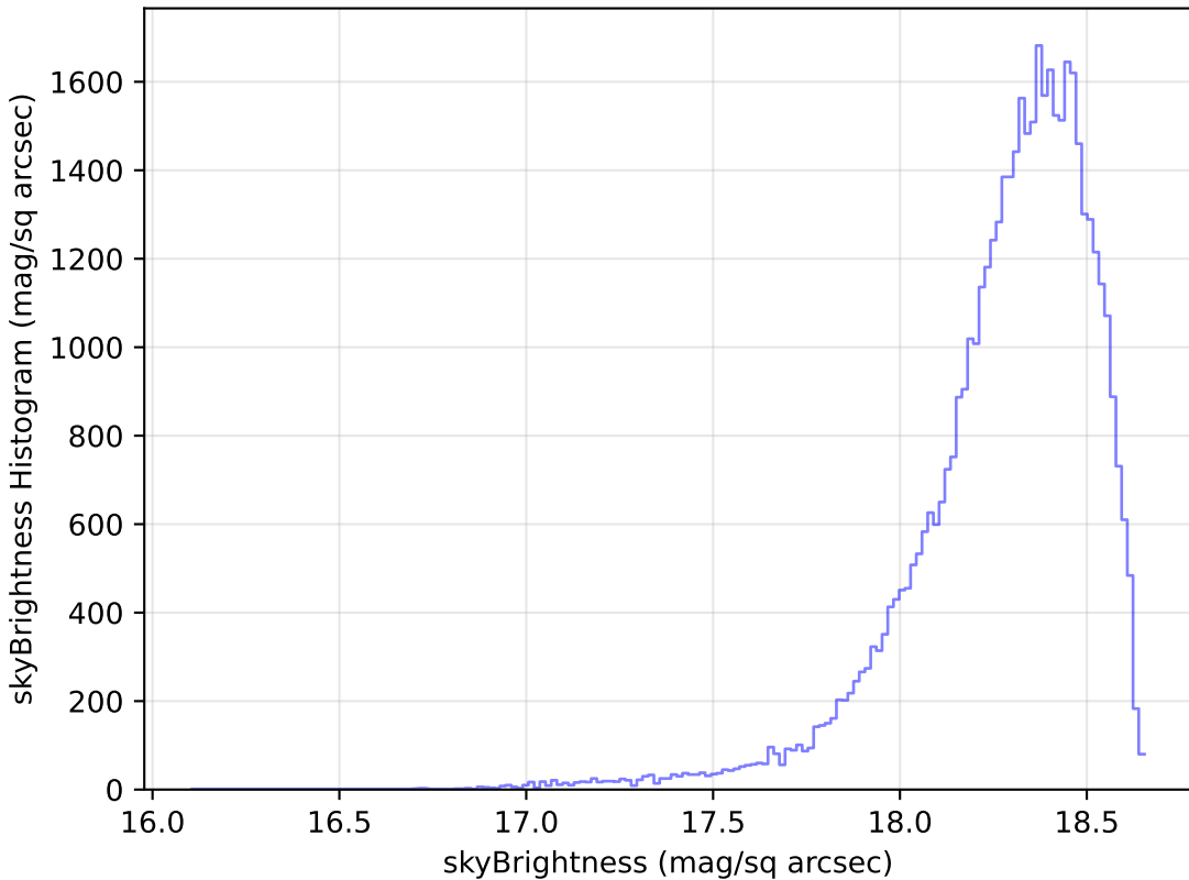
baseline_v3.2_10yrs Yr 1 y band: skyBrightness Histogram
