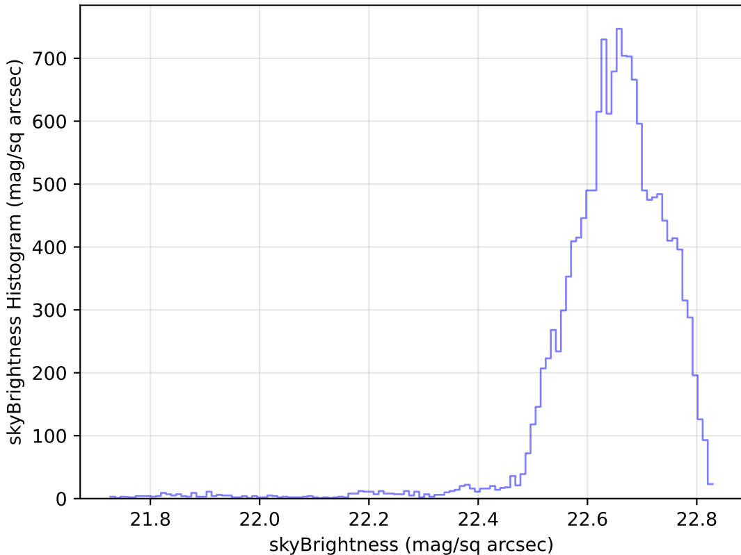
baseline_v3.2_10yrs Yr 1 u band: skyBrightness Histogram
