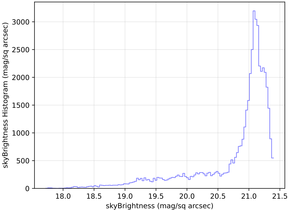
baseline_v3.2_10yrs Yr 1 r band: skyBrightness Histogram
