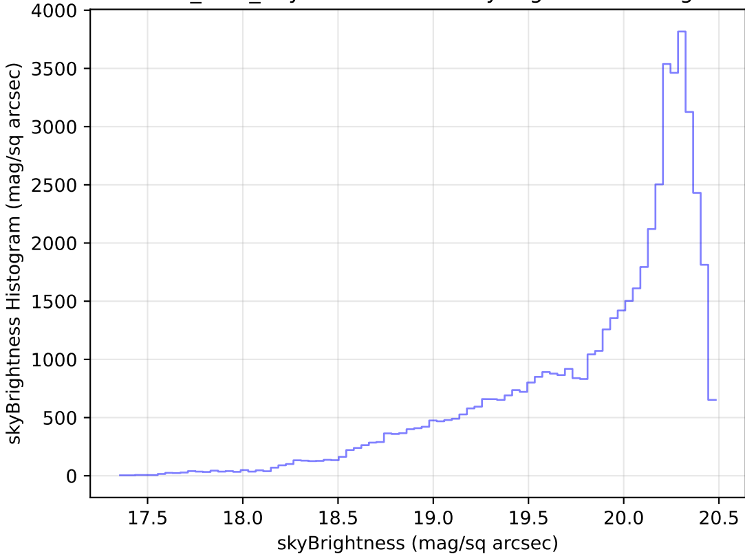
baseline_v3.2_10yrs Yr 1 i band: skyBrightness Histogram
