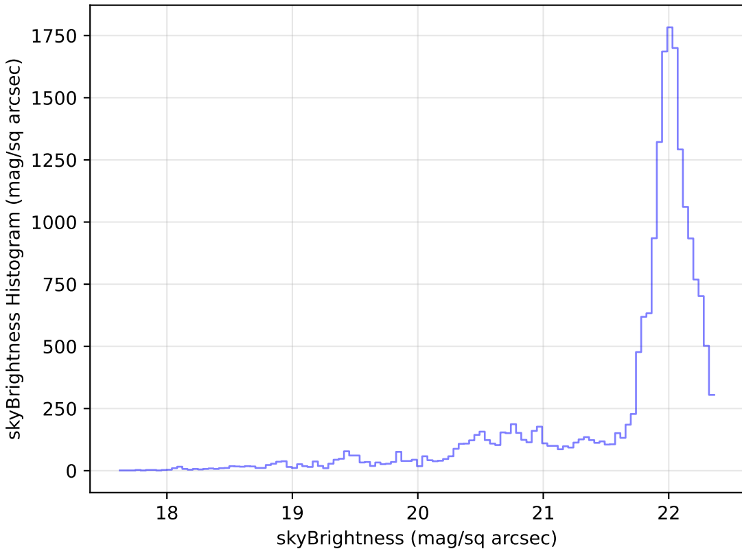
baseline_v3.2_10yrs Yr 1 g band: skyBrightness Histogram
