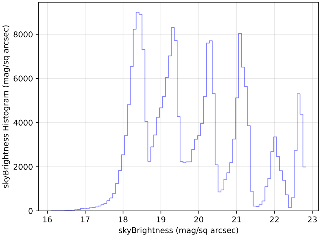
baseline_v3.2_10yrs Yr 1 all bands: skyBrightness Histogram
