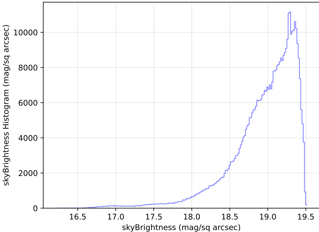
baseline_v3.2_10yrs WFD z band: skyBrightness Histogram
