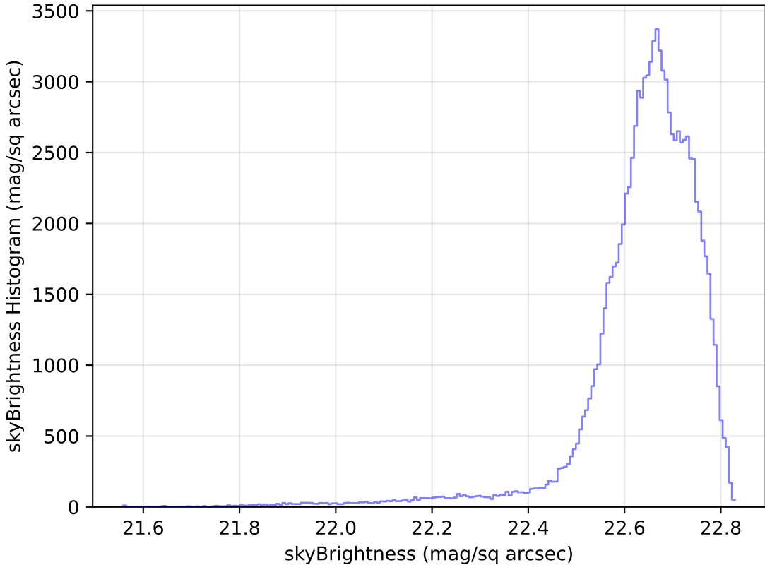
baseline_v3.2_10yrs WFD u band: skyBrightness Histogram
