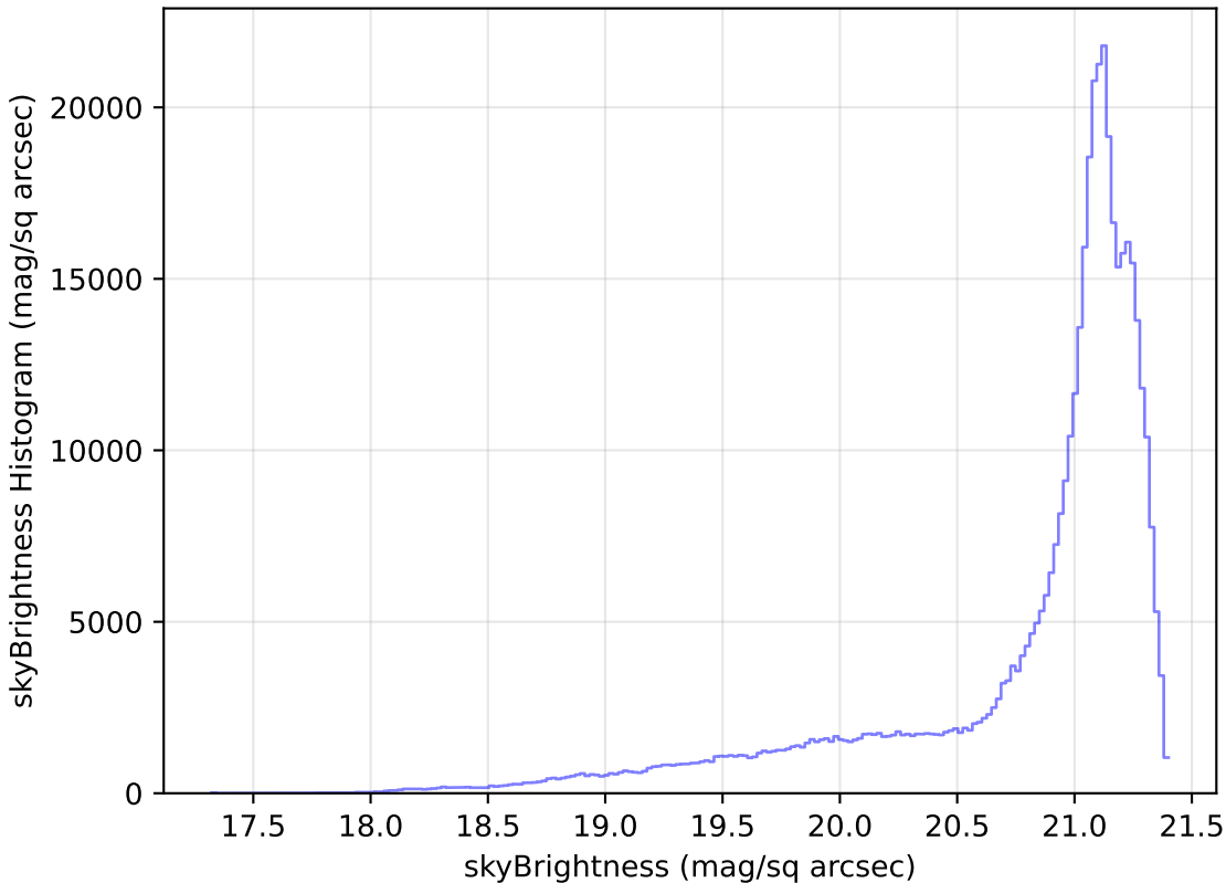
baseline_v3.2_10yrs WFD r band: skyBrightness Histogram
