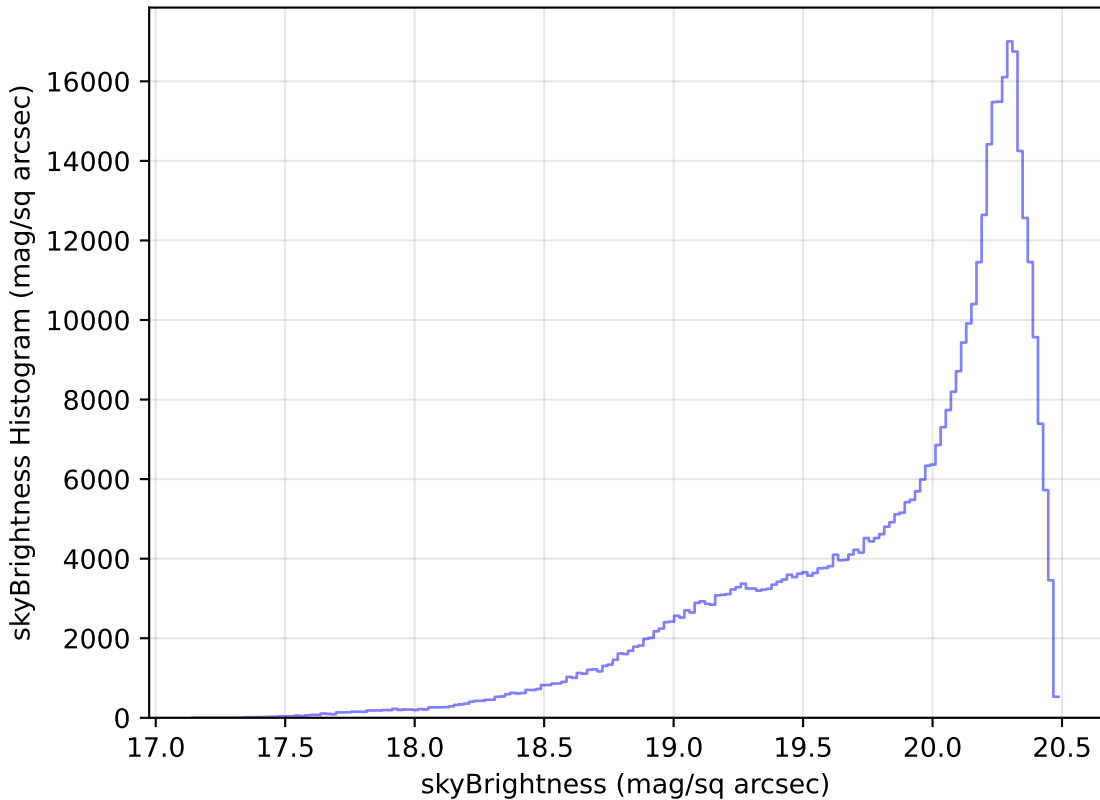
baseline_v3.2_10yrs WFD i band: skyBrightness Histogram
