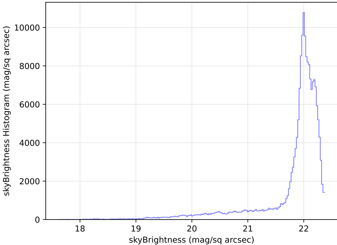
baseline_v3.2_10yrs WFD g band: skyBrightness Histogram
